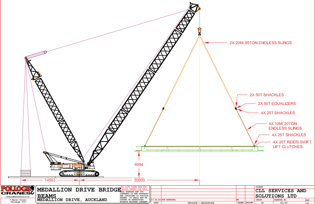
BRIDGE BEAM MO8- LIFT PLAN SIDE ELEVATION
